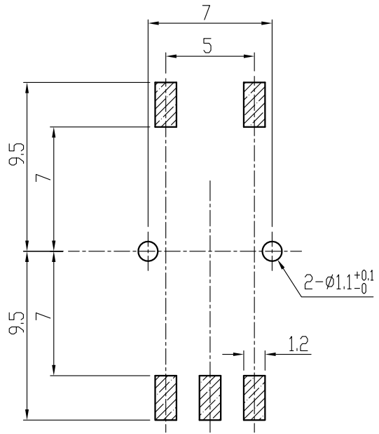
P.C.B.MOUNTING DETAIL
